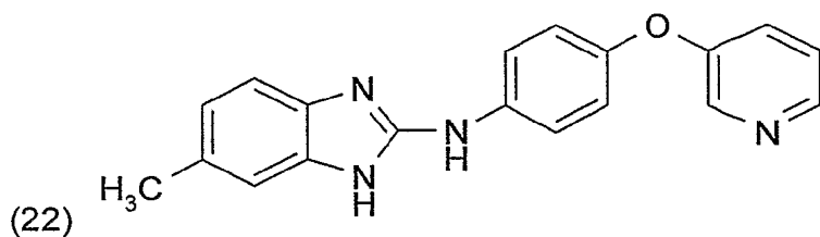
(6-Methyl-1H-benzimidazol-2-yl)-[4-(pyridin-3-yloxy)-phenyl]-amin
